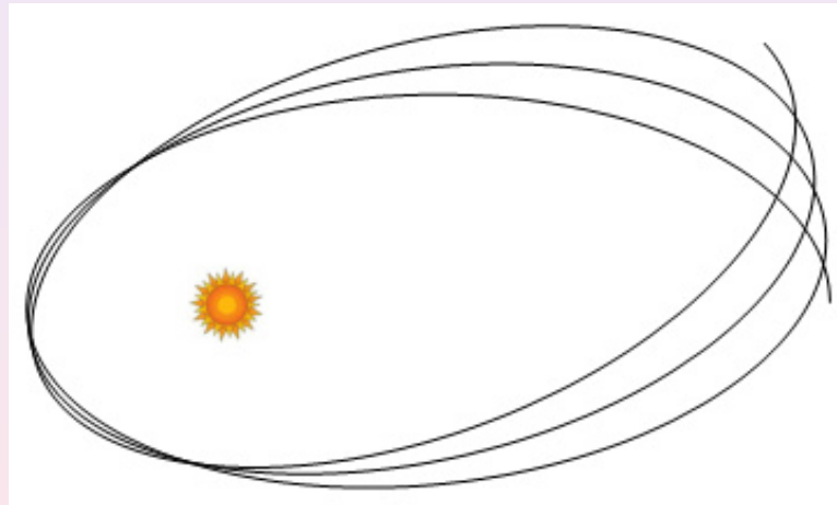
Perihelion of mercury
