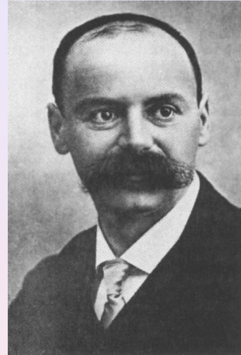
Schwarzschild
