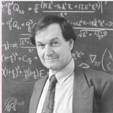
Penrose
